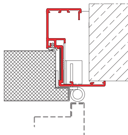
→ hybrid frame – hinge side view, 3D adjustable hinge
