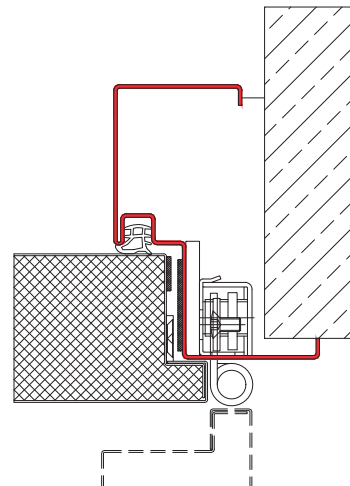
→ hybrid frame – hinge side view, 3D adjustable hinge
