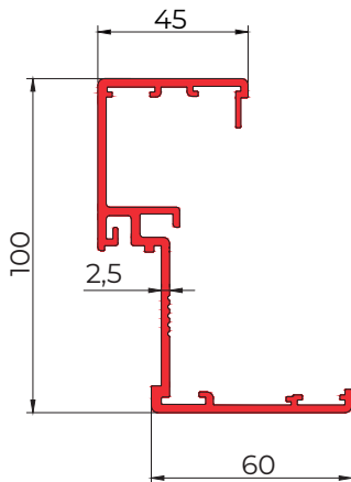
→ hybrid aluminium frame – general view
